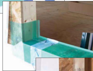
Secure with Nails or Staples
