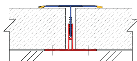
Two-piece Flex-Tite system
